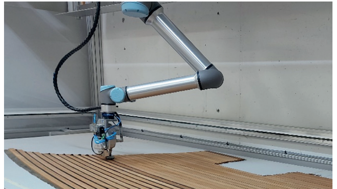
Collaborative machining, handling and (dis)assembling
