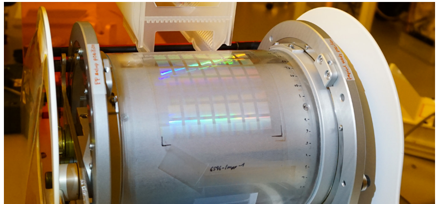
Nanostructures replicated with Step&Repeat and STENSBERG Roll-to-Plate NIL
