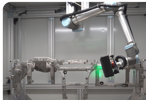
Complete solution for the inspection of aluminum structural components
