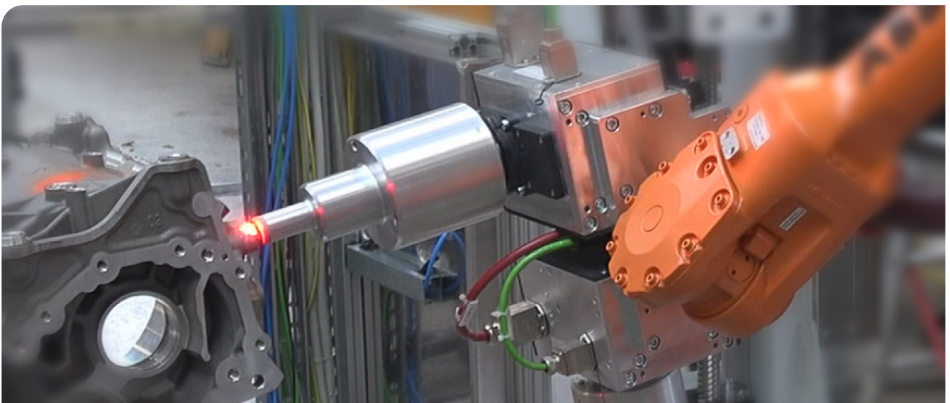
D20-F rotating sensor during hole inspection
