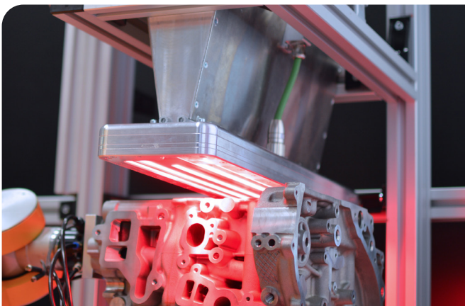
Engine block inspection with TPScan Sensor 400
