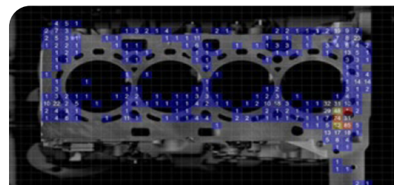
Intuitive display of defect frequencies from a series of measurements
