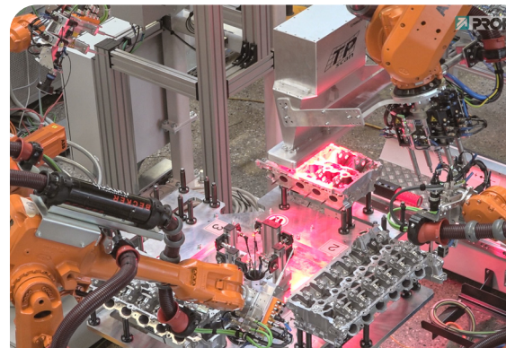
Complete solution for the inspection of engine blocks
