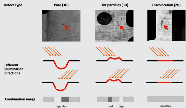
Robust differentiation between 3D and 2D effects
