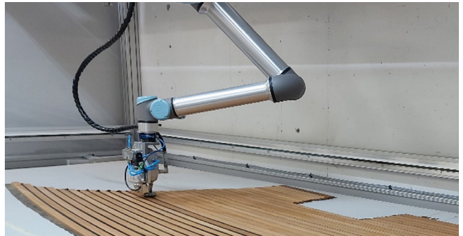
Collaborative machining, handling and (dis)assembling
