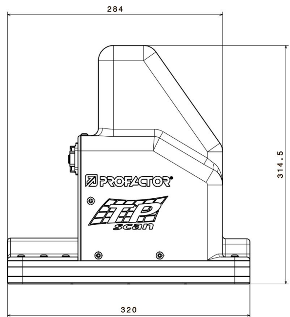
TPScan Sensor 180
